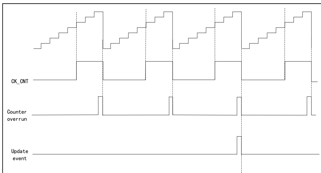
Figure 25 Timing Diagram of Count-up Mode when Setting REPCNT=2
