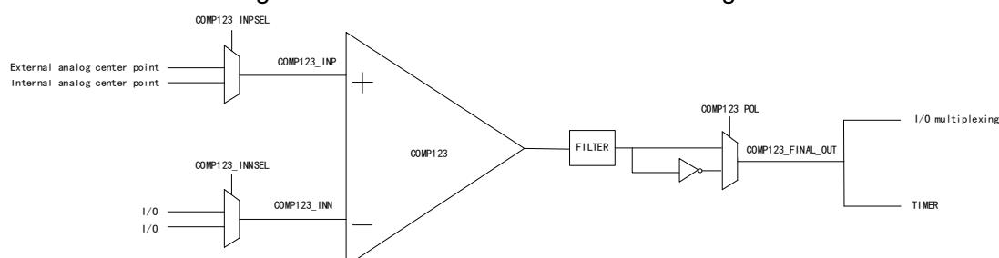
Figure 108 COMP1/2/3 Structure Block Diagram
