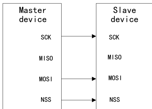
Figure 97 Connection in Simplex Mode(the master only transmit and the slave receive)
