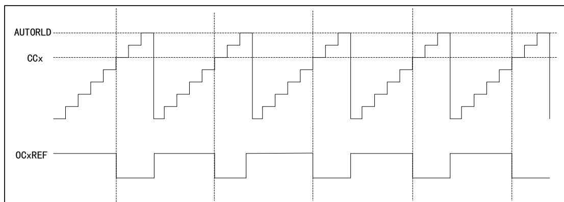
Figure 60 Timing Diagram of PWM1 Count-down Mode
