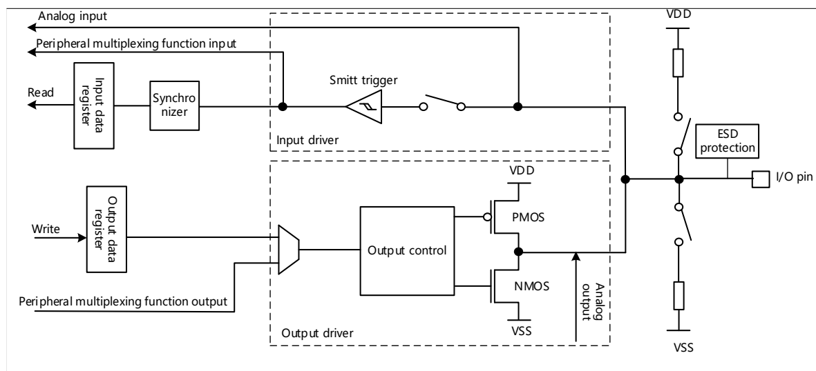
Figure 15 GPIO Structure Block Diagram
