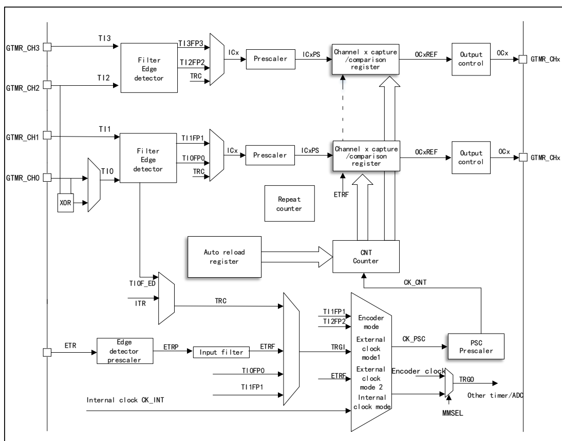
Figure 39 Structure Block Diagram
