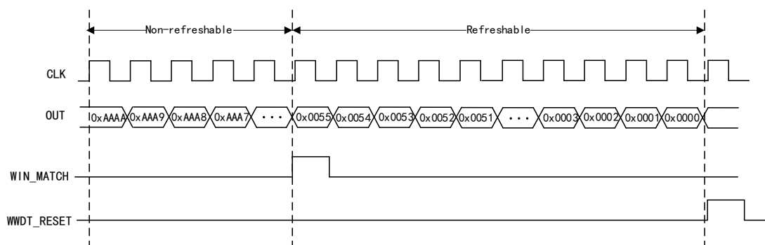
Figure 70 Timing Diagram
