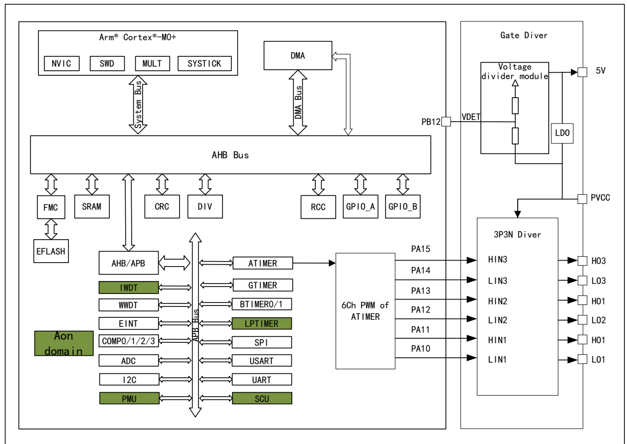
Figure 5 System Architecture Block Diagram
