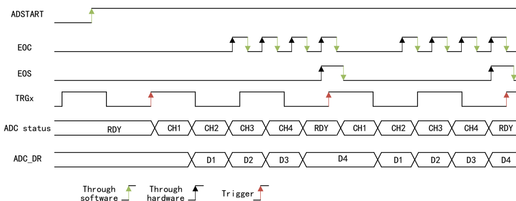
Figure 103 Single sequence conversion, hardware trigger
